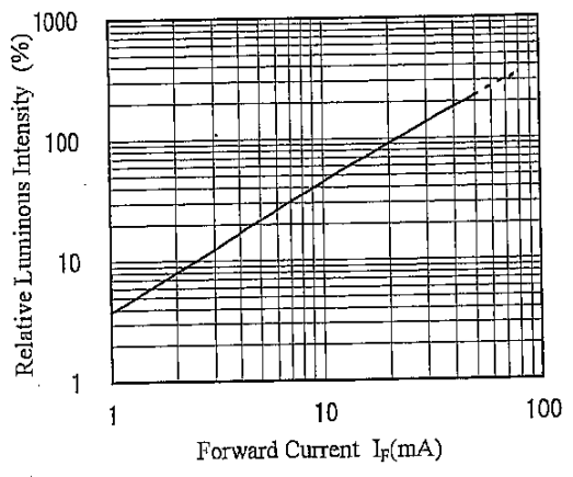
Relative Luminous Intensity vs. Forward Current ( T_c=25^\circ\text{C} )
