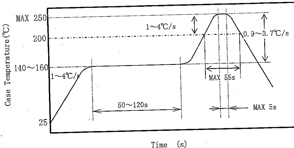
Fig. Reflow soldering temperature profile
