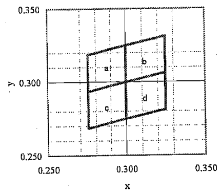
6-4-2 chromaticity rank graph (Tolerance : x,y: ±0.02)
