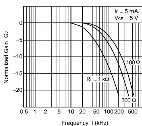
FREQUENCY RESPONSE
