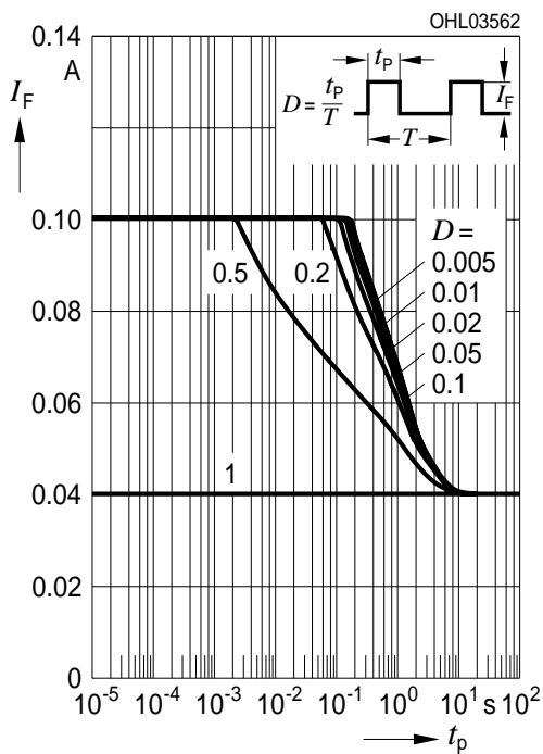
Zulässige Impulsbelastbarkeit Permissible Pulse Handling Capability Duty cycle D = \text{parameter} , T_A = 85^\circ\text{C} I_F = f(t_p) ; red (1 Chip on)
