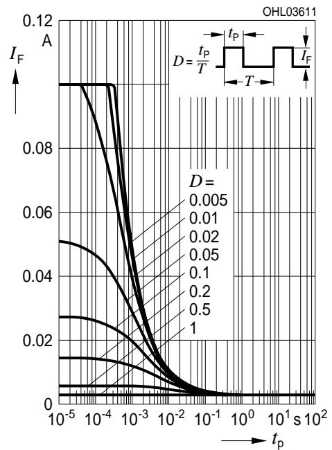
Zulässige Impulsbelastbarkeit I_F = f(t_p) Permissible Pulse Handling Capability Duty cycle D = parameter, T_A = 85\text{ °C} blue, true green
