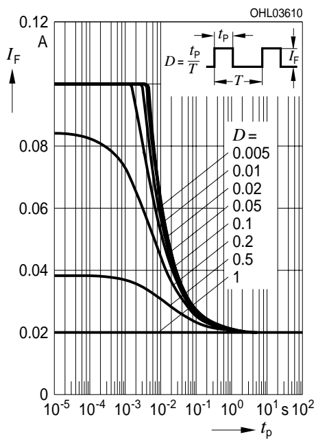
Zulässige Impulsbelastbarkeit I_F = f(t_p) Permissible Pulse Handling Capability Duty cycle D = parameter, T_A = 25\text{ °C} blue, true green
