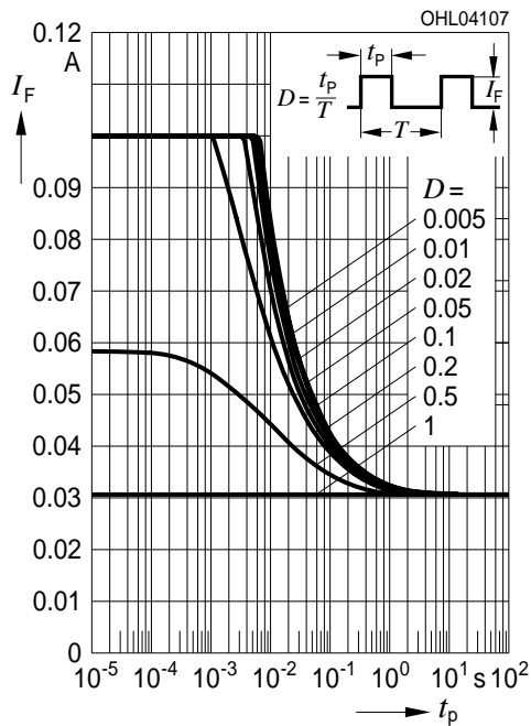
Zulässige Impulsbelastbarkeit I_F = f(t_p) Permissible Pulse Handling Capability Duty cycle D = parameter, T_A = 25\text{ °C} blue, true green
