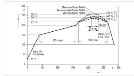
REFLOW PROFILE FOR ROHS COMPLIANT PARTS
