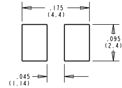
RECOMMENDED SOLDER PAD LAYOUT
