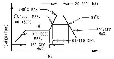
RECOMMENDED REFLOW SOLDERING PROFILE FOR 80/20 Sn/Pb PARTS
