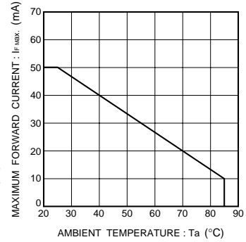
Fig.10 Maximum forward current vs. ambient temperature (Derating)
