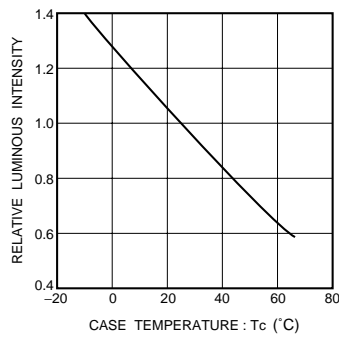
Fig.6 Luminous intensity vs. case temperature
