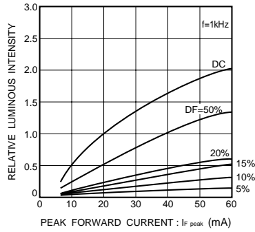
Fig.9 Luminous intensity vs. peak forward current
