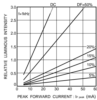
Fig.15 Luminous intensity vs. peak forward current
