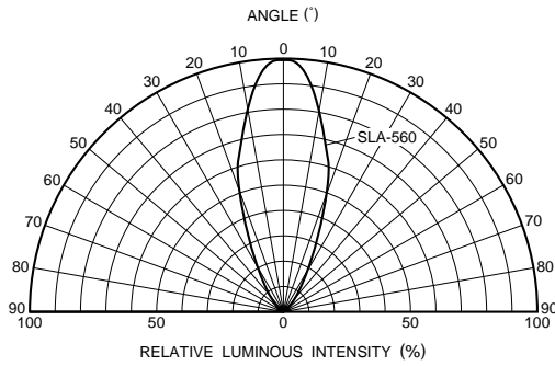
Fig.2 SLA-560 Directional pattern
