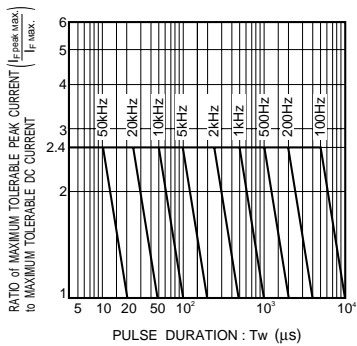
Fig.14 Maximum tolerable peak current vs. pulse duration
