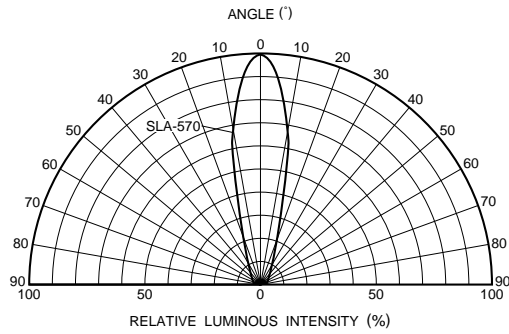
Fig.3 SLA-570 Directional pattern
