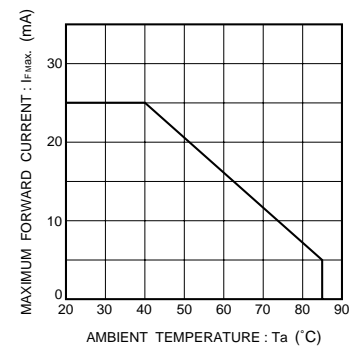
Fig.16 Maximum forward current vs. ambient temperature (Derating)
