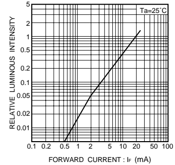
Fig.13 Luminous intensity vs. forward current
