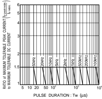
Fig.8 Maximum tolerable peak current vs. pulse duration
