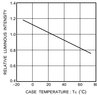
Fig.12 Luminous intensity vs. case temperature
