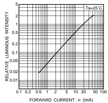
Fig.7 Luminous intensity vs. forward current
