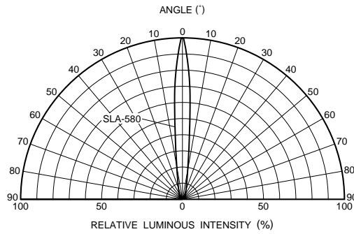
Fig.4 SLA-580 Directional pattern
