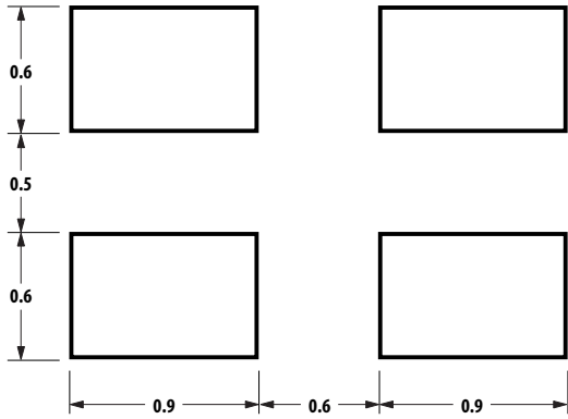
Figure 8. Recommended soldering land pattern.
