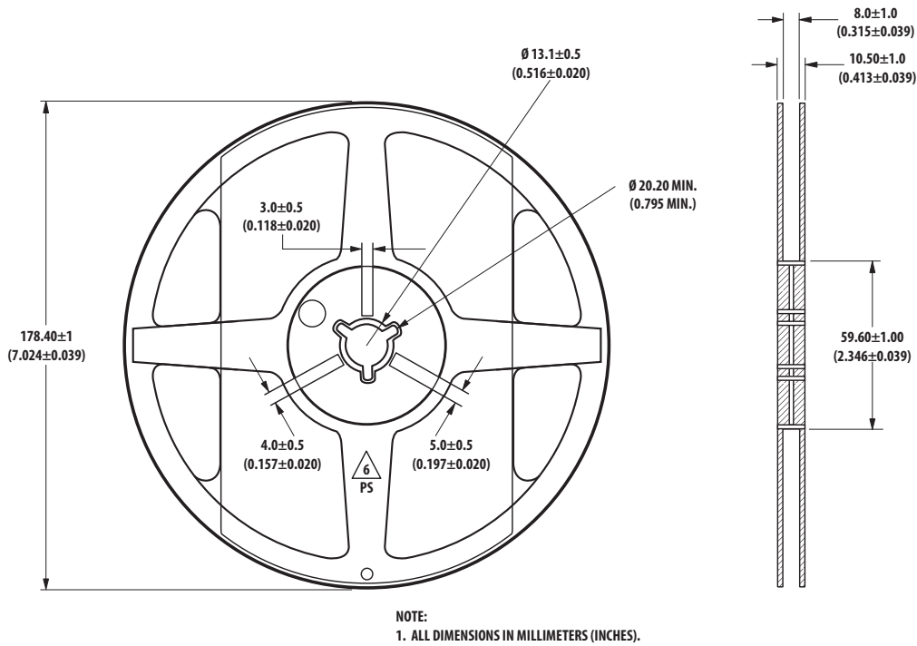
Figure 10. Reel dimensions.
