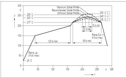
RoHS COMPLIANT REFLOW PROFILE
