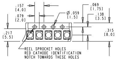
TAPE & REEL CONFIGURATION
