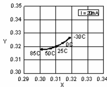
Fig.9 Ambient Temperature vs. Chromaticity Coordinate
