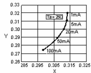
Fig.10 Forward Current vs. Chromaticity Coordinate
