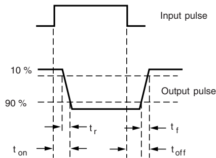
Waveforms
