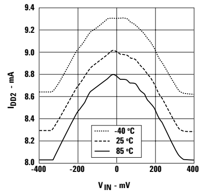
Figure 3. I_{DD2} vs. V_{IN} .
