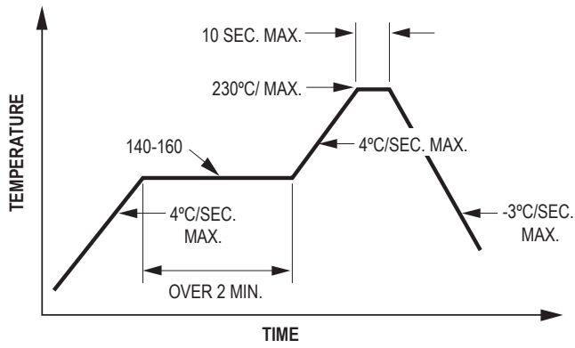
Figure 7a. Recommended reflow soldering profile.
