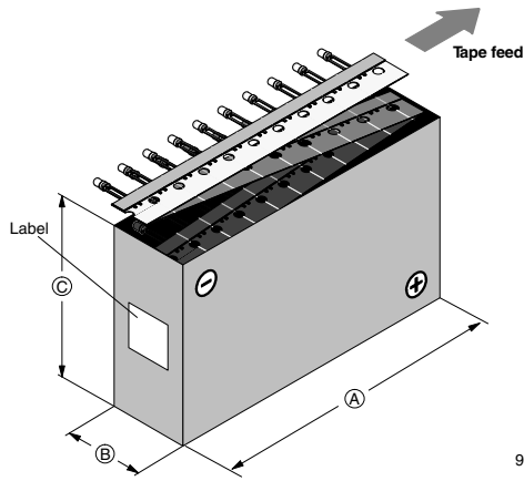
Figure 31. Tape Direction
