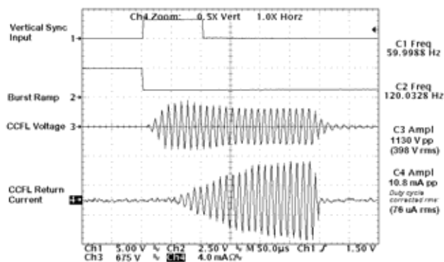
Figure 5 – 2% Burst Duty Cycle (Expanded Time Base)
