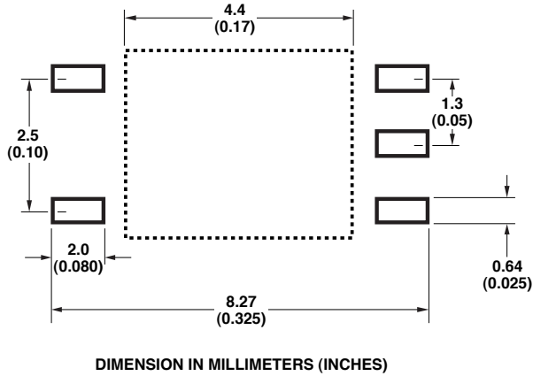
Figure 1.5 Pin SOIC Package (JEDEC M0-155) Device Outline Drawing.
