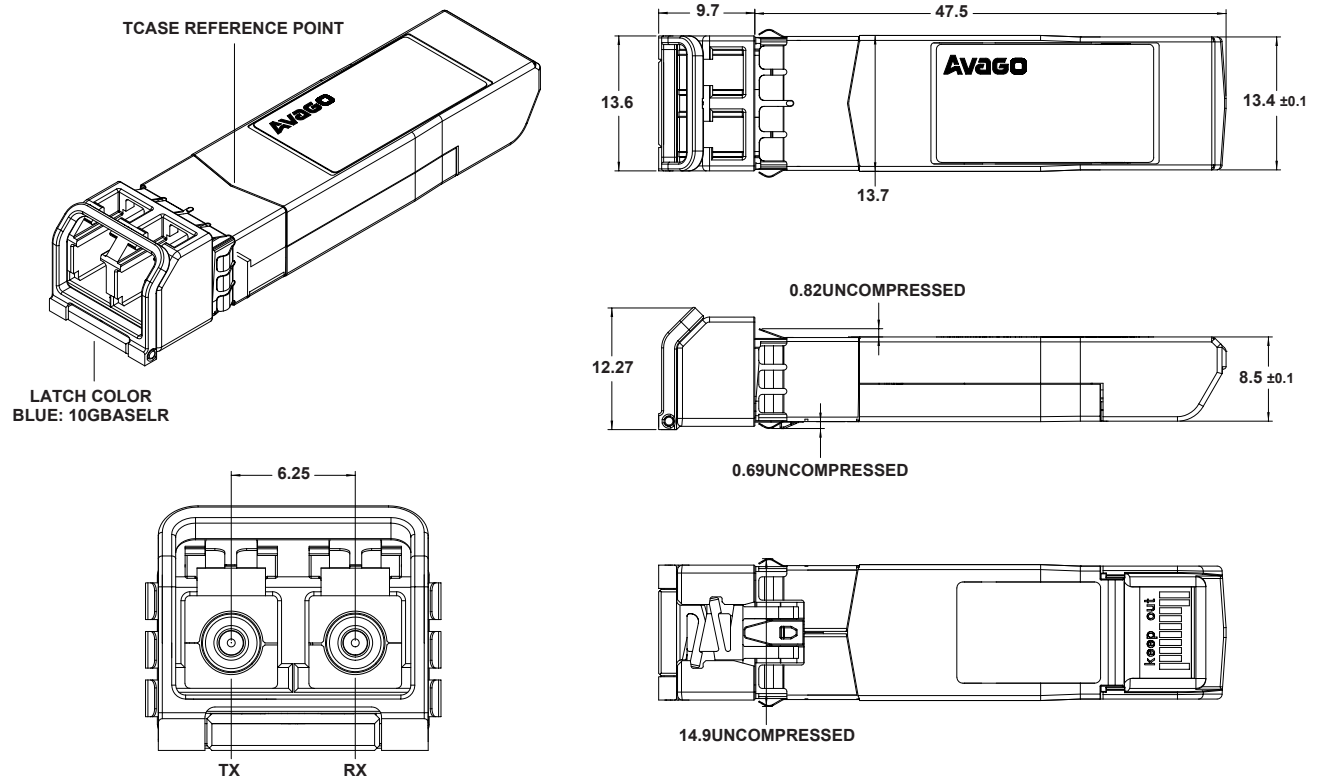
Figure 6. Module drawing
