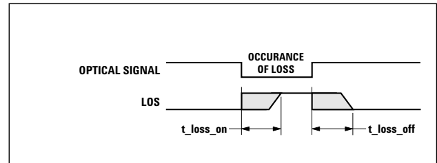
t-loss-on & t-loss-off
