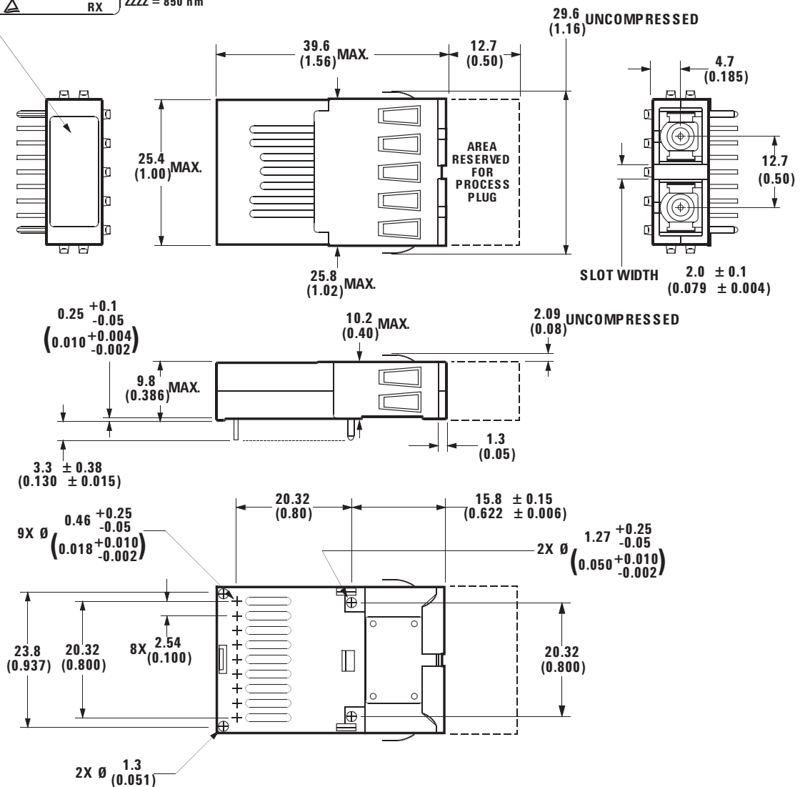
Figure 5. Package outline for AFBR-53B3EZ.
