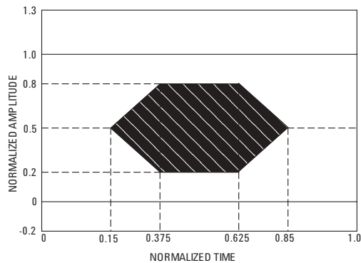
Figure 1. Transmitter optical eye diagram mask.
