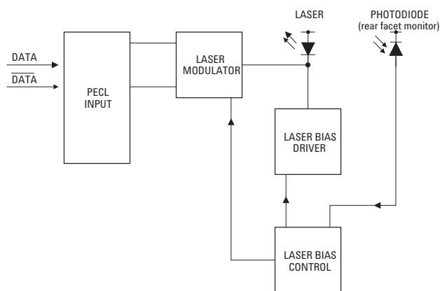
Figure 3 - Simplified Transmitter Schematic
