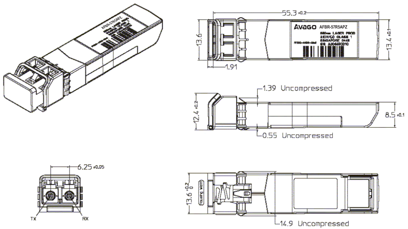
Figure 5. Module drawing
