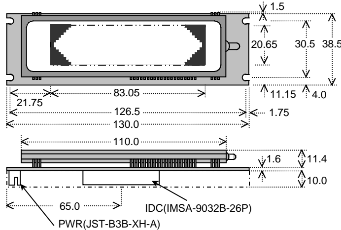
Dimensions in mm & subject to tolerances. Mounting holes 3.5mm dia.
