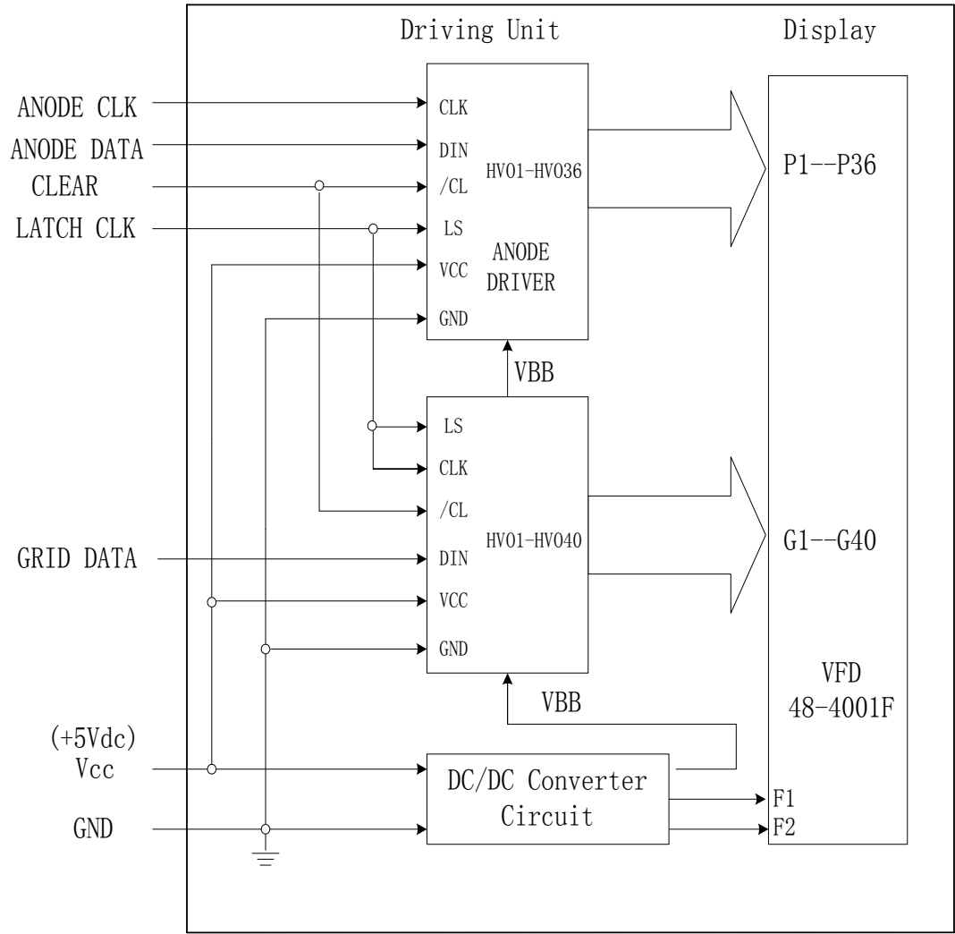
Fig-3. VFD Module System Block Diagram
