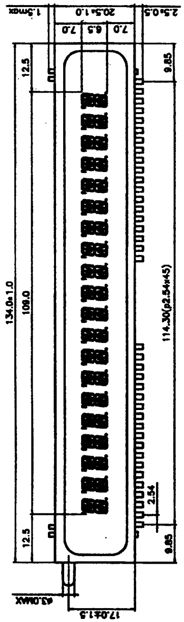
Outline Drawing (Unit:mm)
