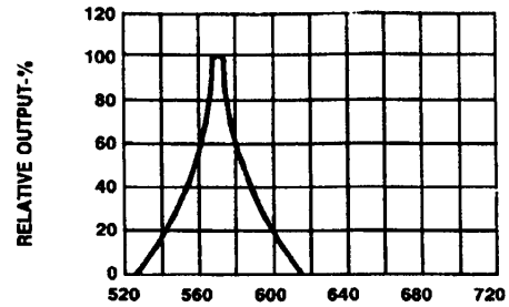
WAVELENGTH ( \lambda )-nm Fig.2 SPECTRAL RESPONSE
