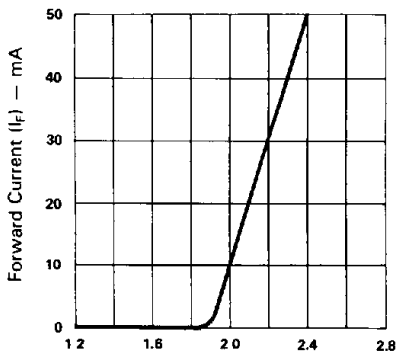
Fig. 1 FORWARD CURRENT I_F Vs FORWARD VOLTAGE.
