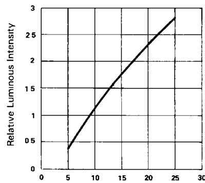
Fig. 3 RELATIVE, LUMINOUS INTENSITY I_v Vs FORWARD CURRENT ( I_F PER SEGMENT)
