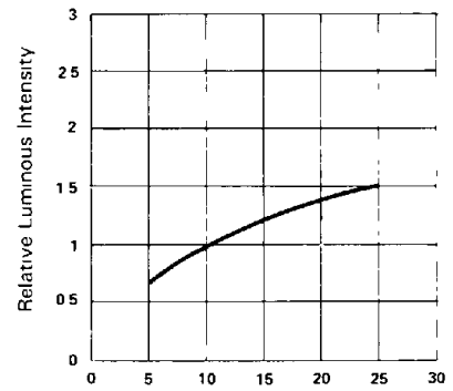
Fig 3 RELATIVE, LUMINOUS INTENSITY Vs FORWARD CURRENT ( I_F PER SEGMENT)
