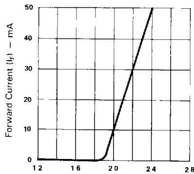
Fig 1 FORWARD CURRENT I_F Vs. FORWARD VOLTAGE V_F
