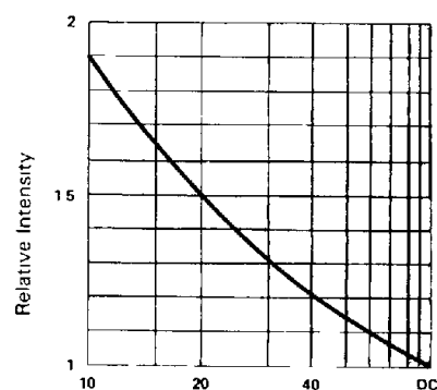
Fig 6 LUMINOUS INTENSITY I_v Vs DUTY CYCLE % (AVERAGE I_F = 10\text{mA} PER SEGMENT)
