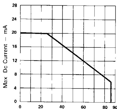
Fig 4 MAX ALLOWABLE DC CURRENT PER SEGMENT Vs AMBIENT TEMPERATURE
