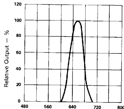
Wavelength ( \lambda ) — nm Fig 2 SPECTRAL RESPONSE
