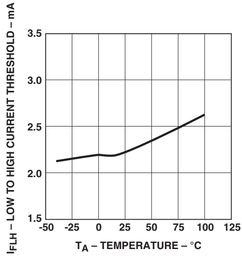
Figure 9. I_{FLH} vs. Temperature.
