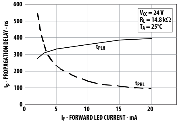
Figure 13b. Typical Propagation Delay vs. Supply Current (ACPL-054L)
