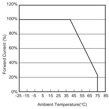
Fig.7 Derating
