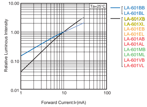
Fig.2 Relative Luminous Intensity - Forward Current
