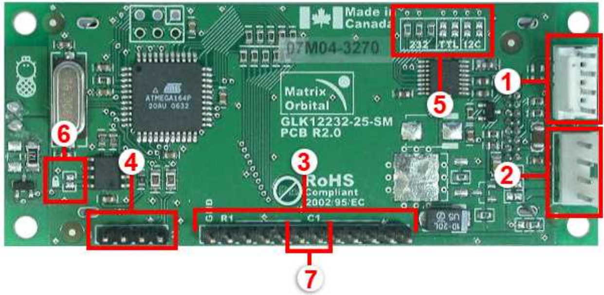
Figure 10: GLK12232-25-SM
