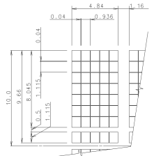
DOT DETAIL (SCALE 5:1)
