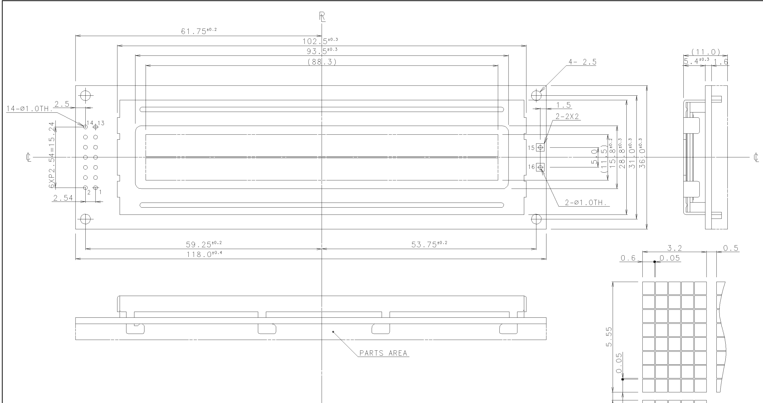
DOT DETAIL : SCALE 10/1
