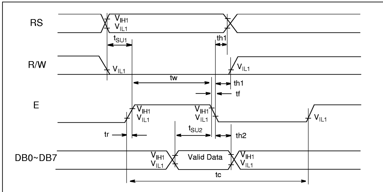
Figure 2: The bus timing diagram for write mode.
