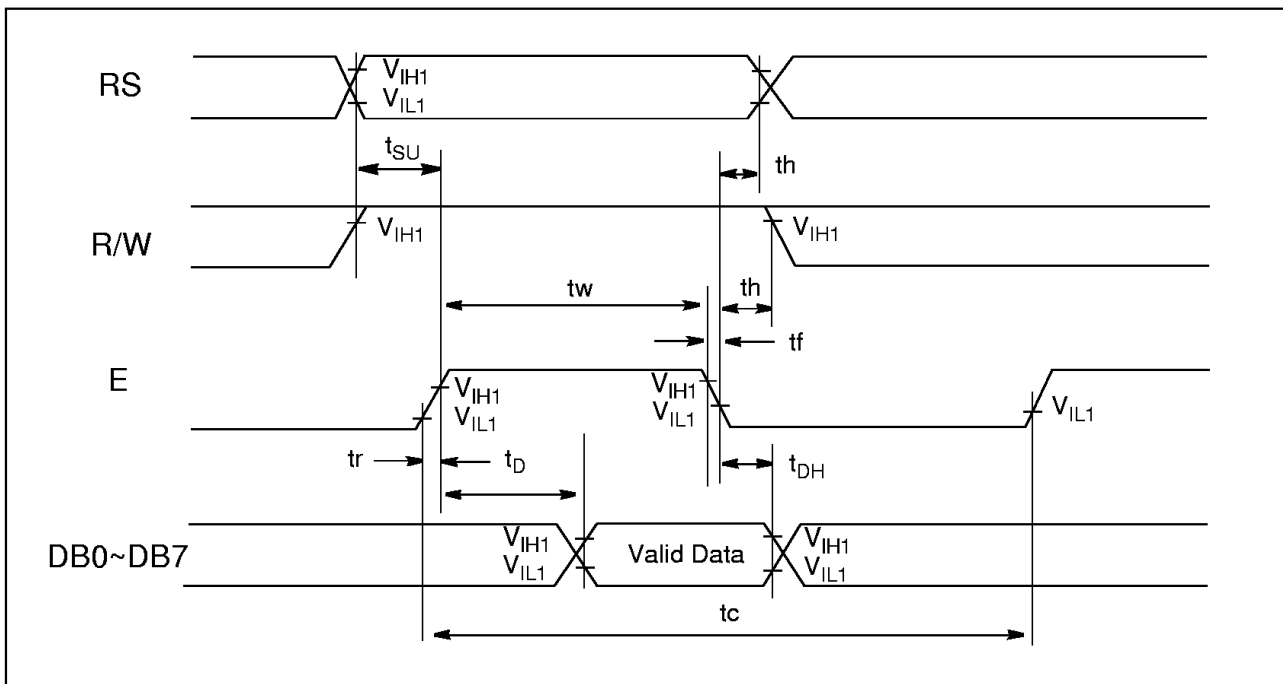
Figure 3: The bus timing diagram for read mode.
