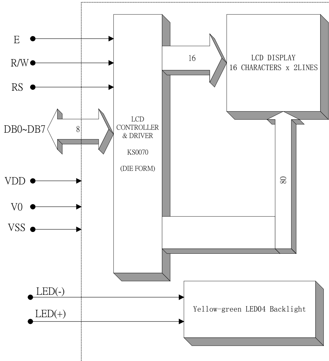
Figure 1(B): Block diagram
