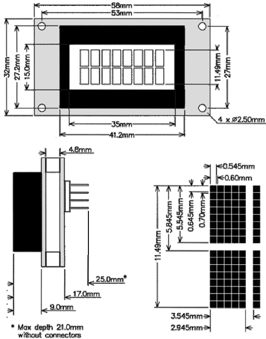
Figure 7-1 Physical Layout
