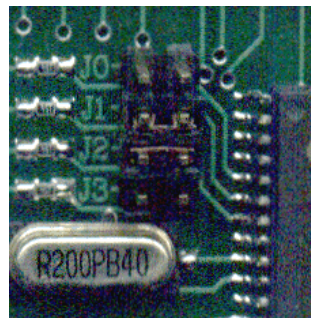
Figure 2-9 RS-232 jumpers
