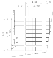
DOT DETAIL (SCALE 5:1)
