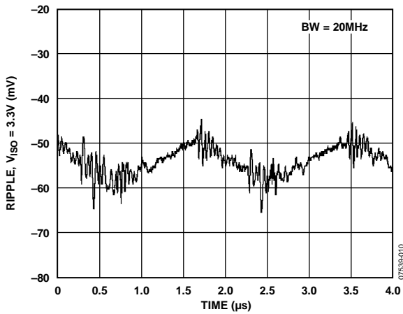
Figure 11. Typical V_{ISO} = 3.3\text{ V} , Output Voltage Ripple at 90% Load
