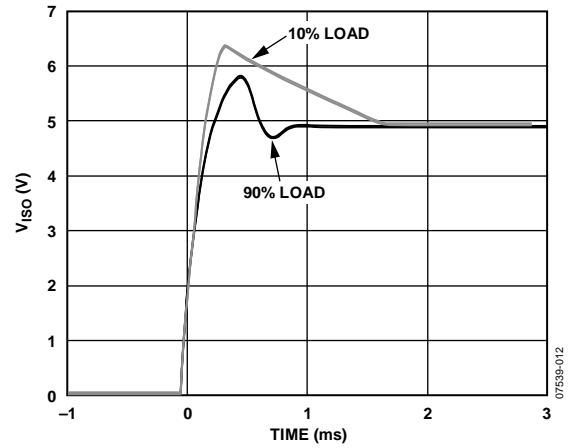
Figure 12. Typical V_{ISO} = 5\text{ V} , Output Voltage Startup Transient at 10% and 90% Load
