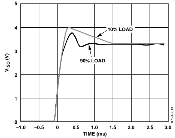
Figure 13. Typical V_{ISO} = 3.3\text{ V} , Output Voltage Startup Transient at 10% and 90% Load
