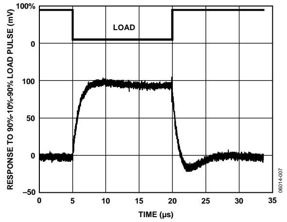
Figure 10. Typical V_{ISO} Transient Load Response, 5 V Output, 90%-10%-90% Pulsed Load, 100 nF Bypass Capacitance vs. Time
