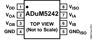
Figure 7. ADuM5242 Pin Configuration
