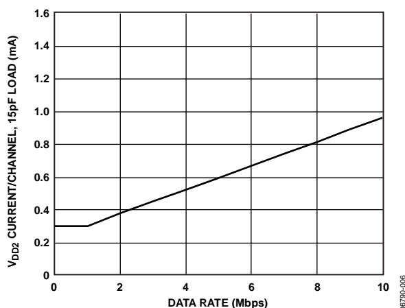
Figure 6. Typical Output Supply Current per Channel vs. Data Rate (15 pF Output Load)
