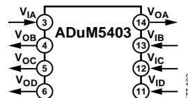
Figure 4. ADuM5403
