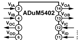
Figure 3. ADuM5402
