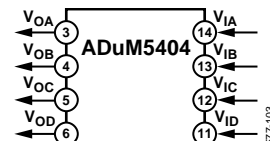
Figure 5. ADuM5404
