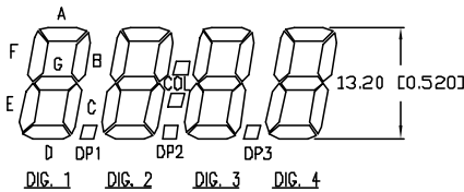
CHARACTER DETAIL
