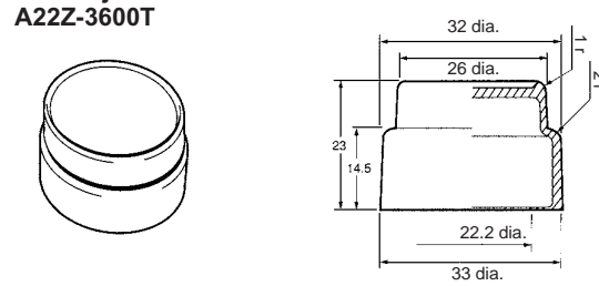
A22Z-3600T
