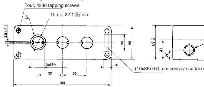
Panel Mounting Hole
