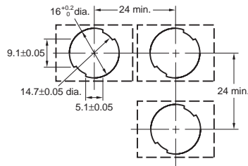
Rectangular A165□-J (Top View)
