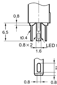
Terminal Arrangement (Bottom View)
