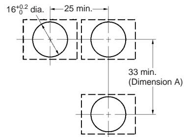
Rectangular A165K□-2S (Top View)
