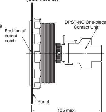
Mounting a 2-pole Switch Unit (See note 5.)
