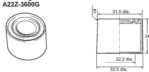
A22Z-3600G
