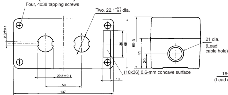
Cable Port Hole (Top View)
