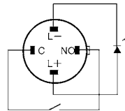
Terminal Arrangement (Bottom View)
