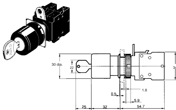
A22E-SK Small Push-lock, Key-reset (30-dia.)
