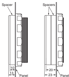
With 1 Spacer
