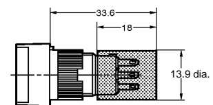
Insulation Cover A3C-3002
