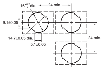
Rectangular A16□-J/M16□-J (Top View)
