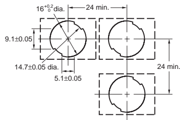
Rectangular A165K-J (Top View)
