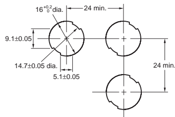
Square A16□-A/M16□-A Round A16□-T/M16□-T (Top View)
