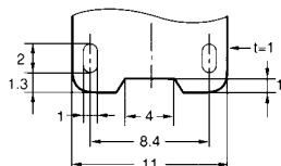
Terminal Hole Dimensions
