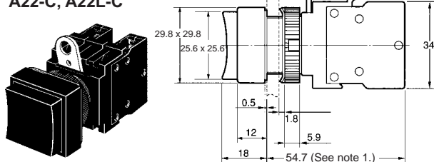
Square/Projection Type A22-C, A22L-C
