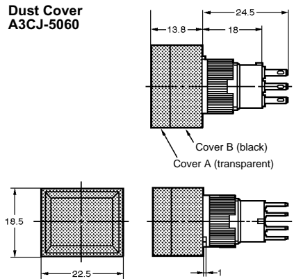
Rectangular
