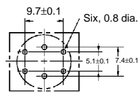
PCB Cutout (bottom view)
