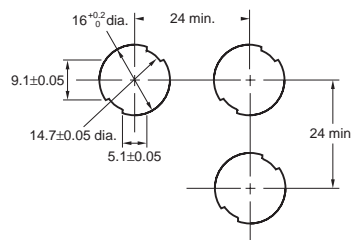
Square A165K-A Round A165K-T (Top View)
