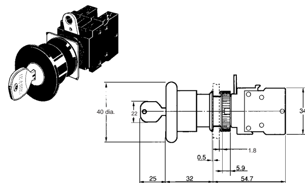
A22E-MK Medium Push-lock, Key-reset (40-dia.)
