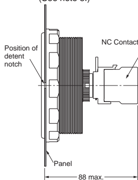
Mounting a 1-pole Switch Unit (See note 5.)
