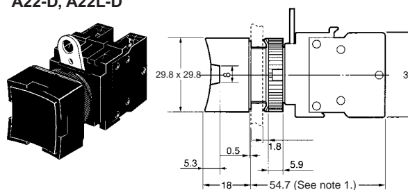
Square/Full-guard Type A22-D, A22L-D
