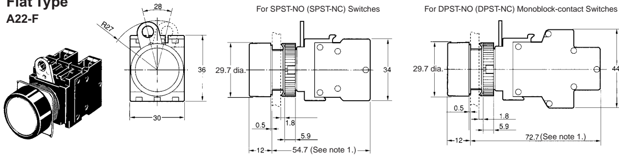
Round/Half-guard Type A22-H, A22L-H
