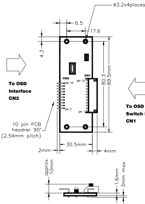
Membrane Interface Board: P/N:416100120-3
