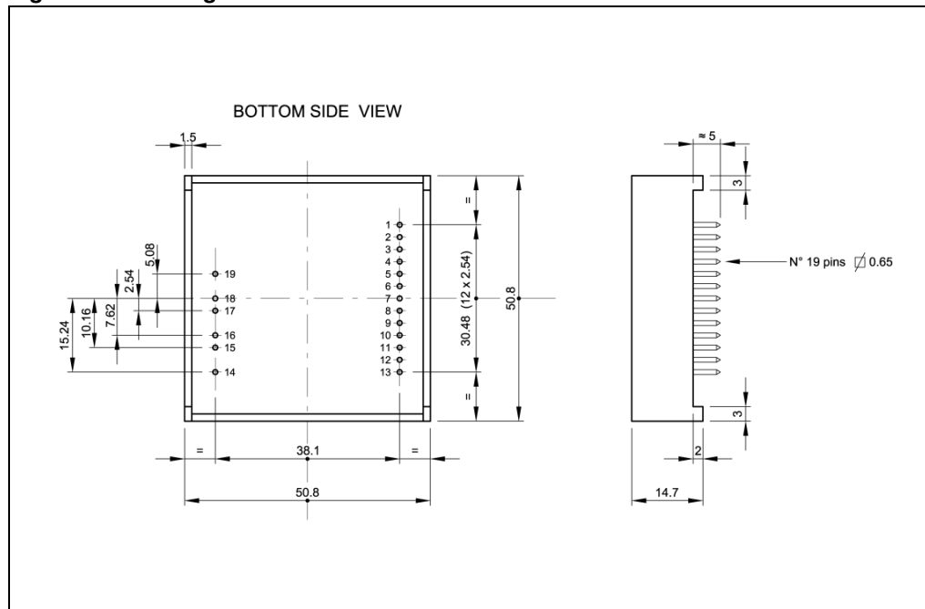
Figure 22. Package dimensions
