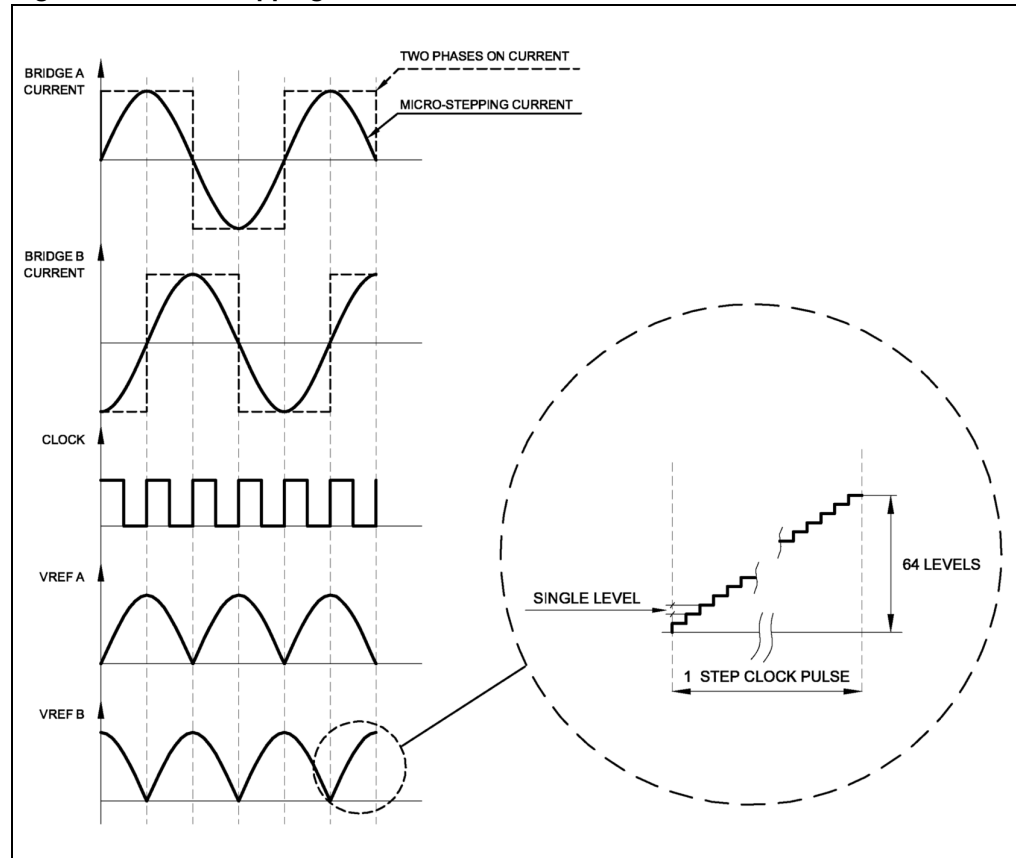
Figure 20. Microstepping
