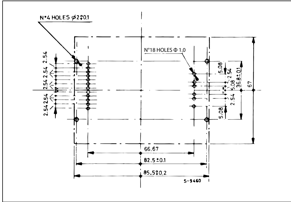
Figure 20. Motherboard layout
