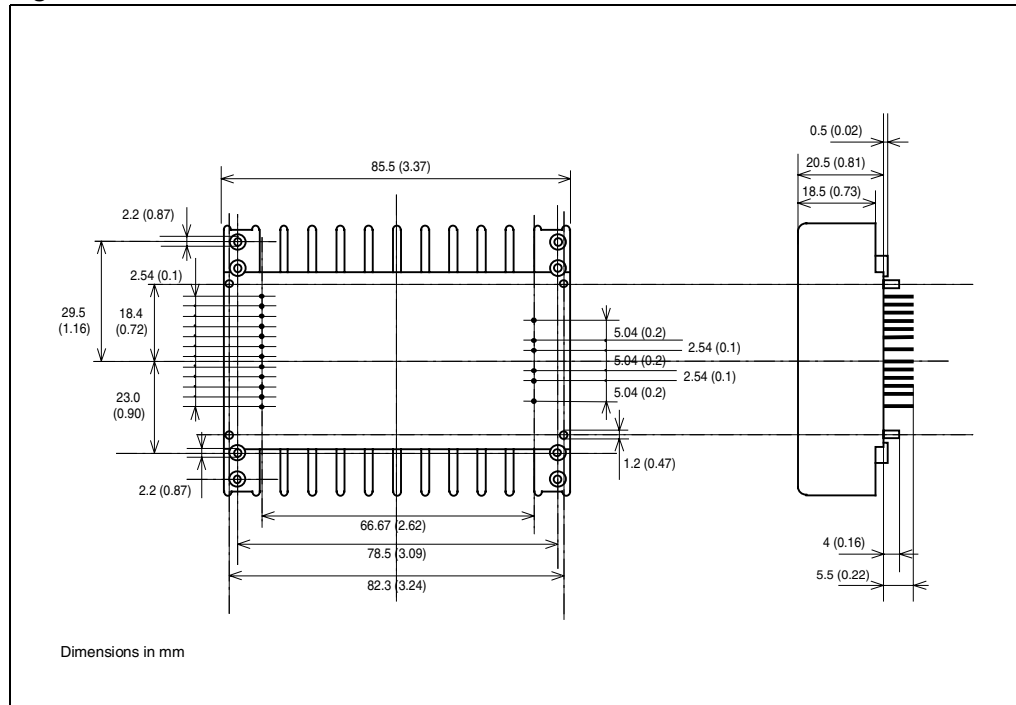
Figure 19. Mechanical data
