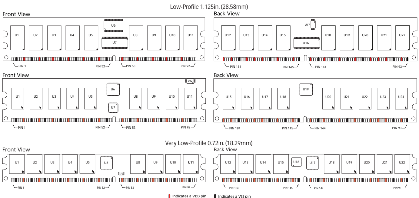
Figure 2: Pin Locations
