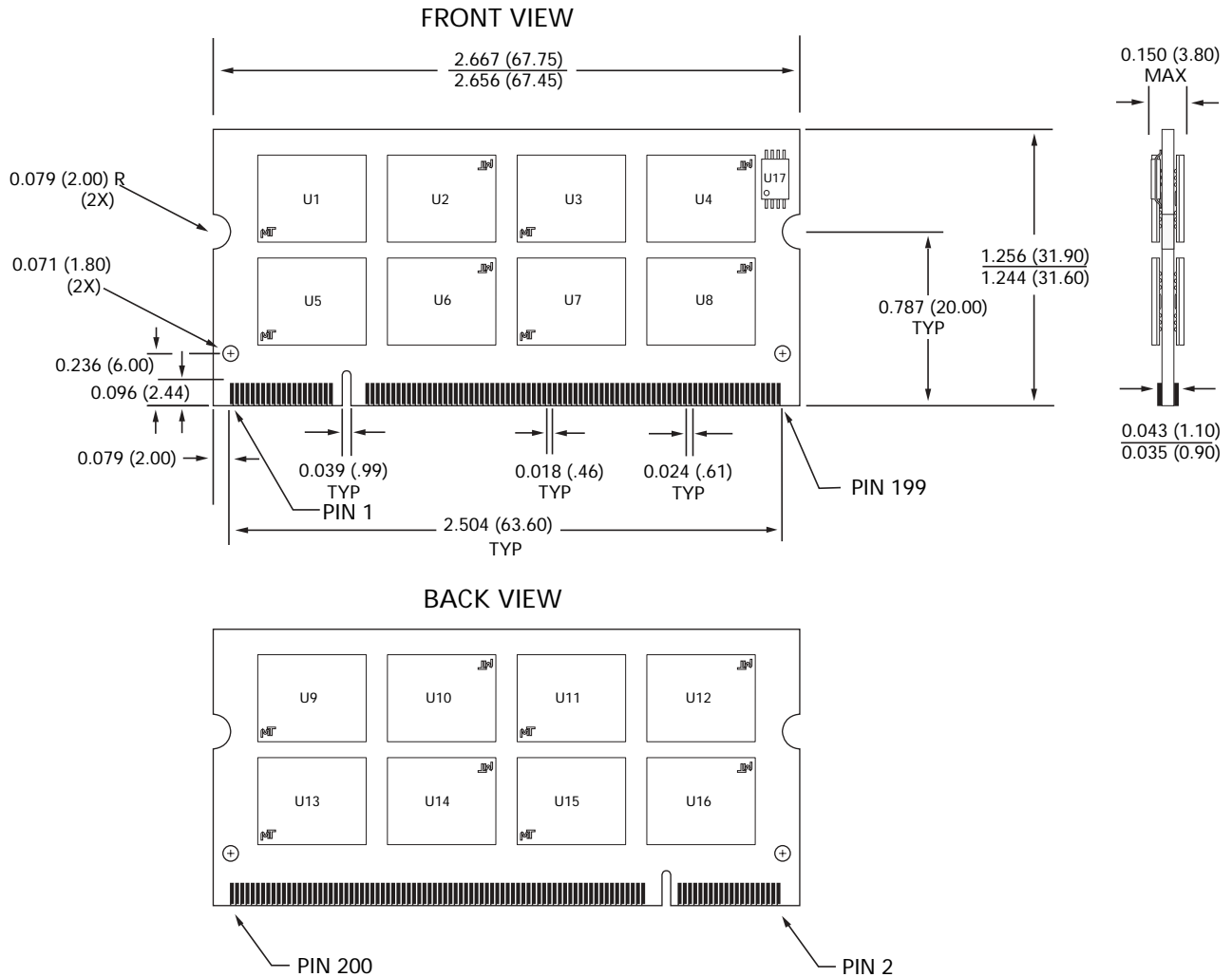
Figure 17: 200-PIN SODIMM Dimensions – 1GB
