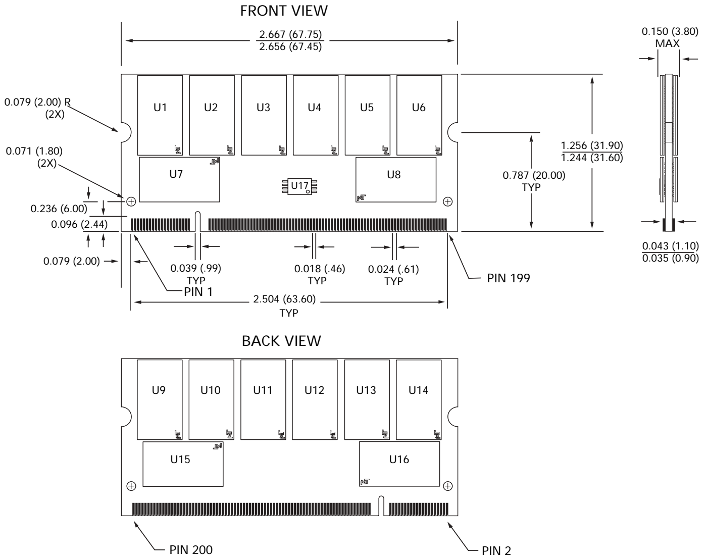
Figure 16: 200-PIN SODIMM Dimensions – 512MB
