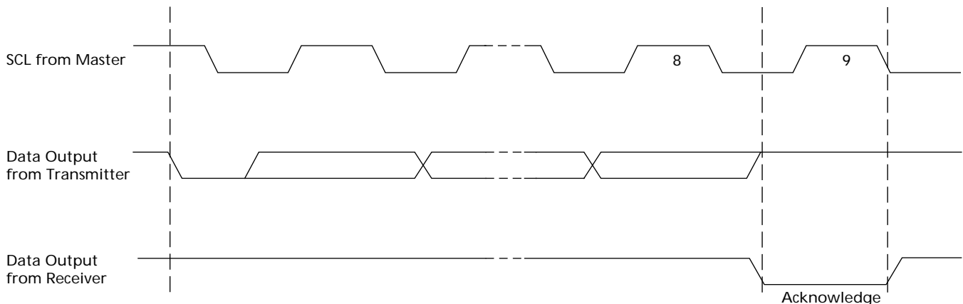
Figure 14: Acknowledge Response From Receiver
