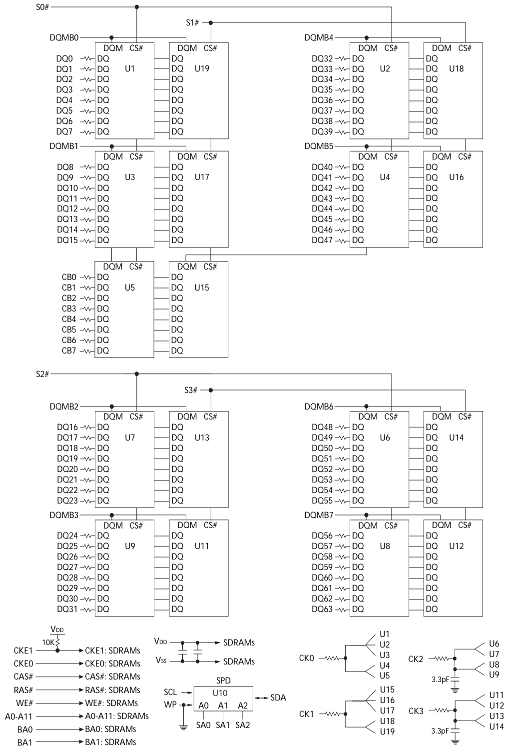
Figure 4: Functional Block Diagram – Dual Rank
