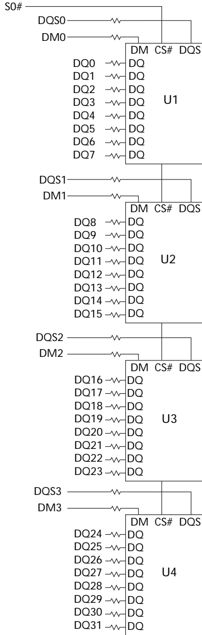
Figure 3: Functional Block Diagram
