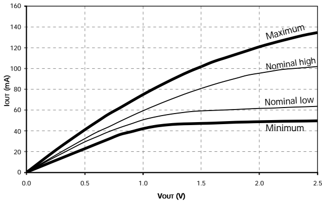
Figure 8: Pull-Down Characteristics
