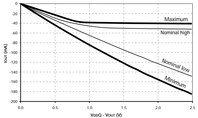
Figure 9: Pull-Up Characteristics
