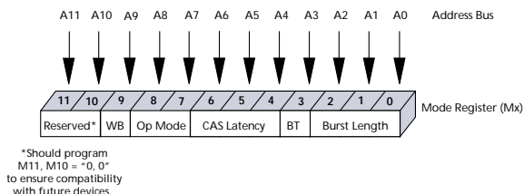
Figure 4: Mode Register Definition Diagram
