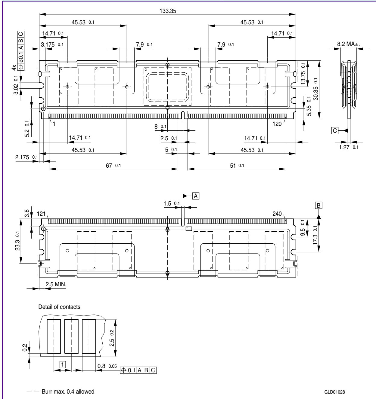
FIGURE 4 Package Outline L-DIM-240-21 with Full Heat Sink
