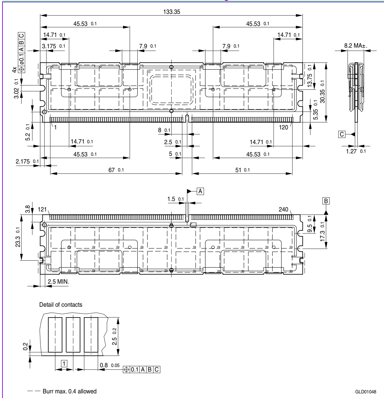
Package Outline L-DIM-240-25 with Full Heat Sink
