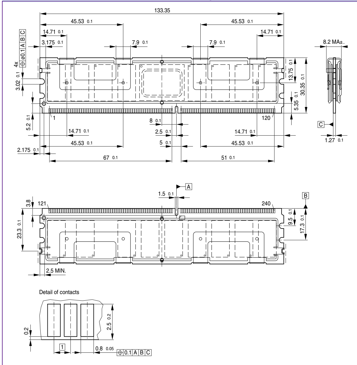
Package Outline L-DIM-240-22 with Full Heat Sink
