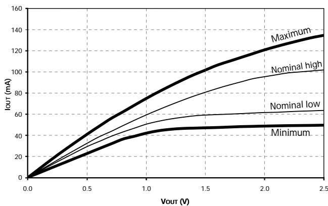
Figure 7: Pull-Down Characteristics
